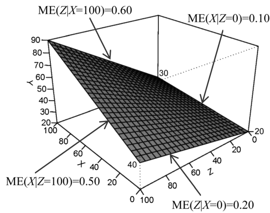
FIGURE 2 Three Conditional Relationships Among X, Z, and Y Consistent with the Plot of ME(X|Z) in Figure 1 (Assuming \beta_X = 0.10 and \beta_{XZ} = 0.004 )
